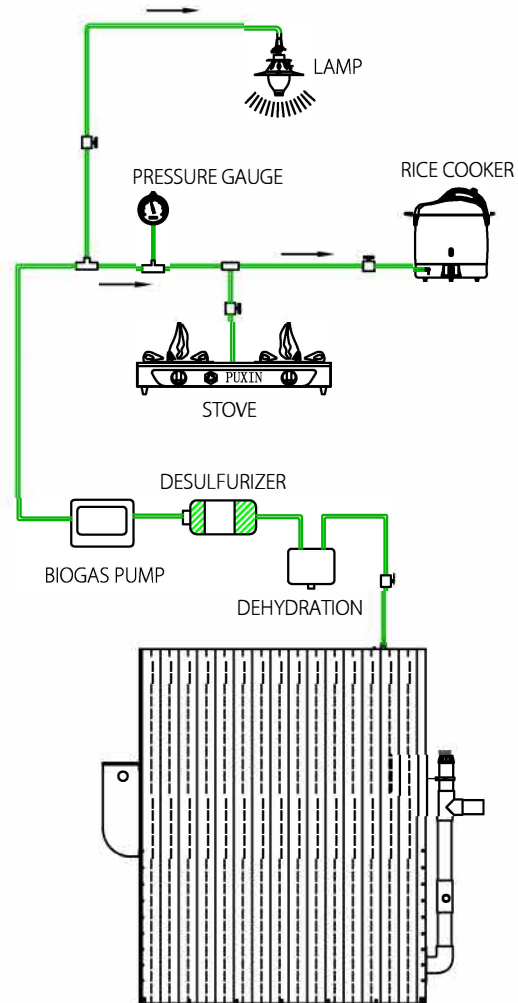
Portable Assembly Biogas System--(Family size)
